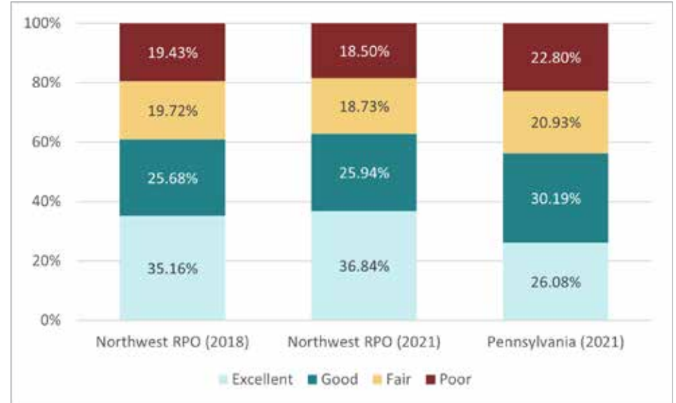
Figure 13: Roadway Condition by IRI Rating, Northwest RPO and Pennsylvania, 2018-2021
