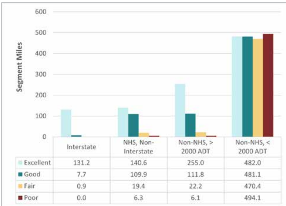
Figure 12: IRI Ratings by Business Plan Network, 2020
